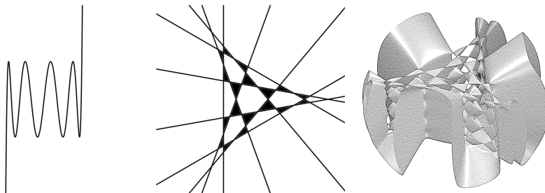
FIGURE 1. For degree d = 9 we show the Tchebychev polynomial T_9(z) , the real folding polynomial F_{\mathbb{R},9}^{A_2}(x, y) associated to the root system A_2 , and the surface \text{Chm}_{\mathbb{R},9}^{A_2}(x, y, z) . The bounded regions in which F_{\mathbb{R},9}^{A_2}(x, y) takes negative values are marked in black.
